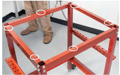
The circles show the mounting hole positions
